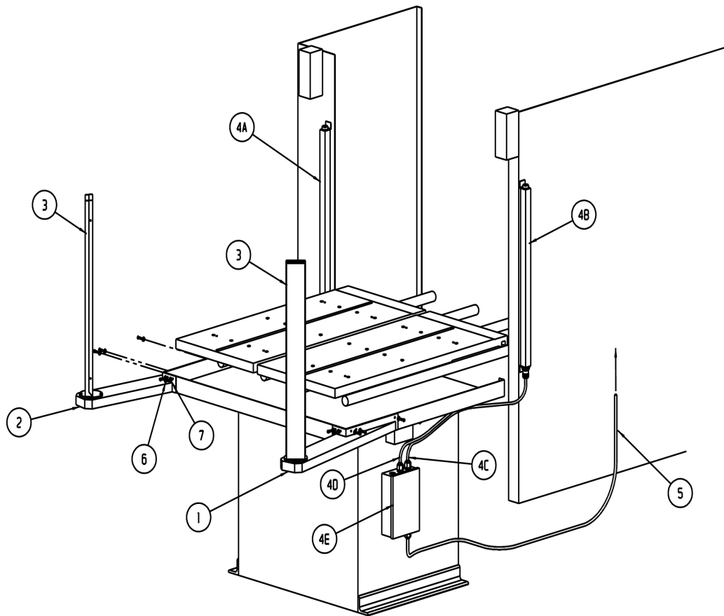
PALLET CHANGER
