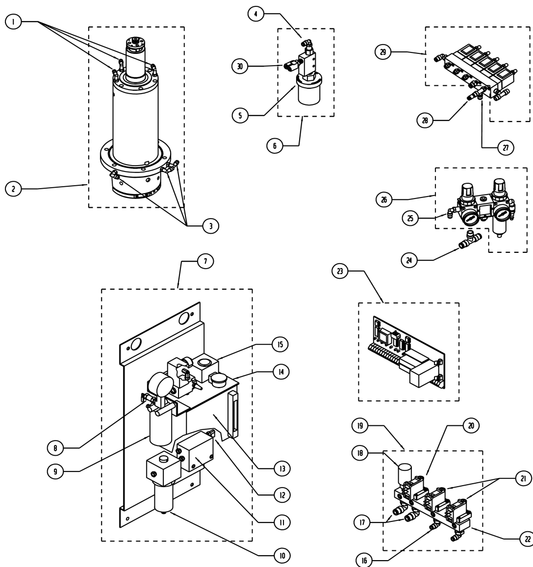
15K AIR/OIL SPIDLE
