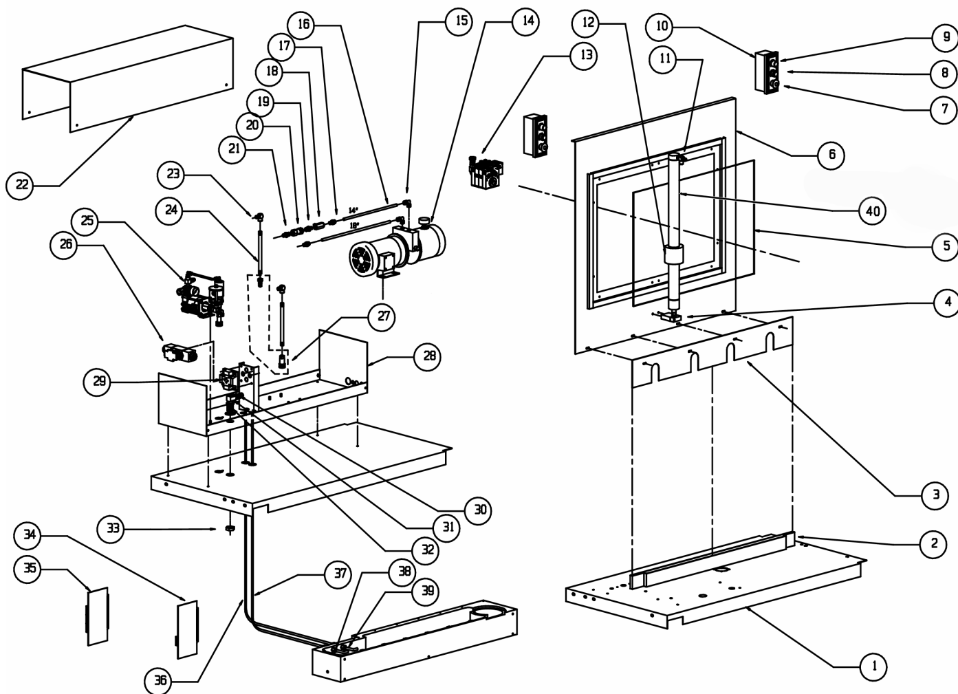
PALLET CHANGER
