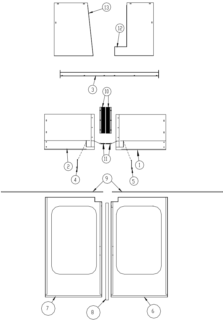
CHAIN HOIST SHEETMETAL 4020S
