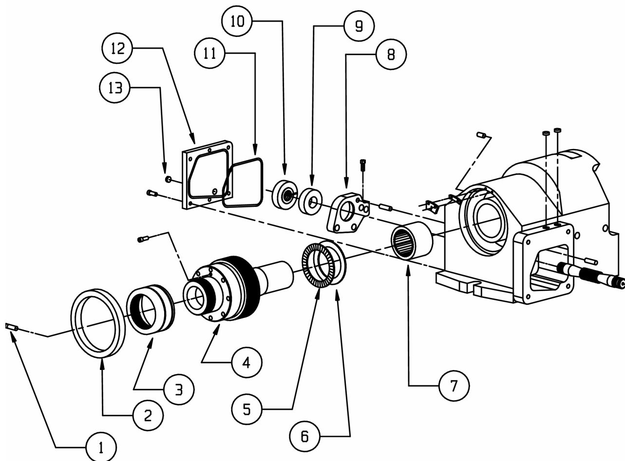
VH5C ROTARY TABLE
