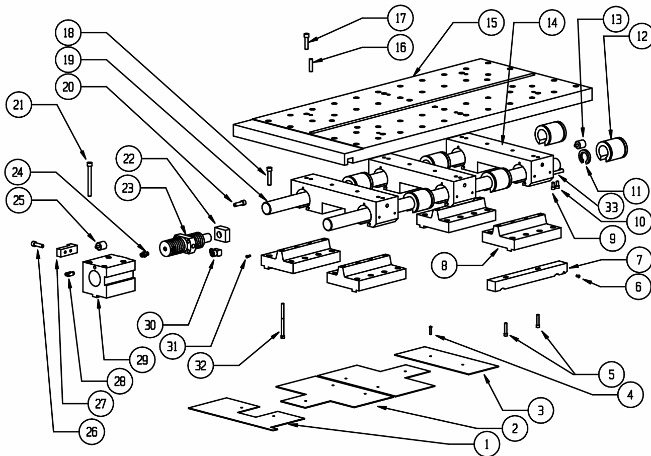
PALLET CHANGER
