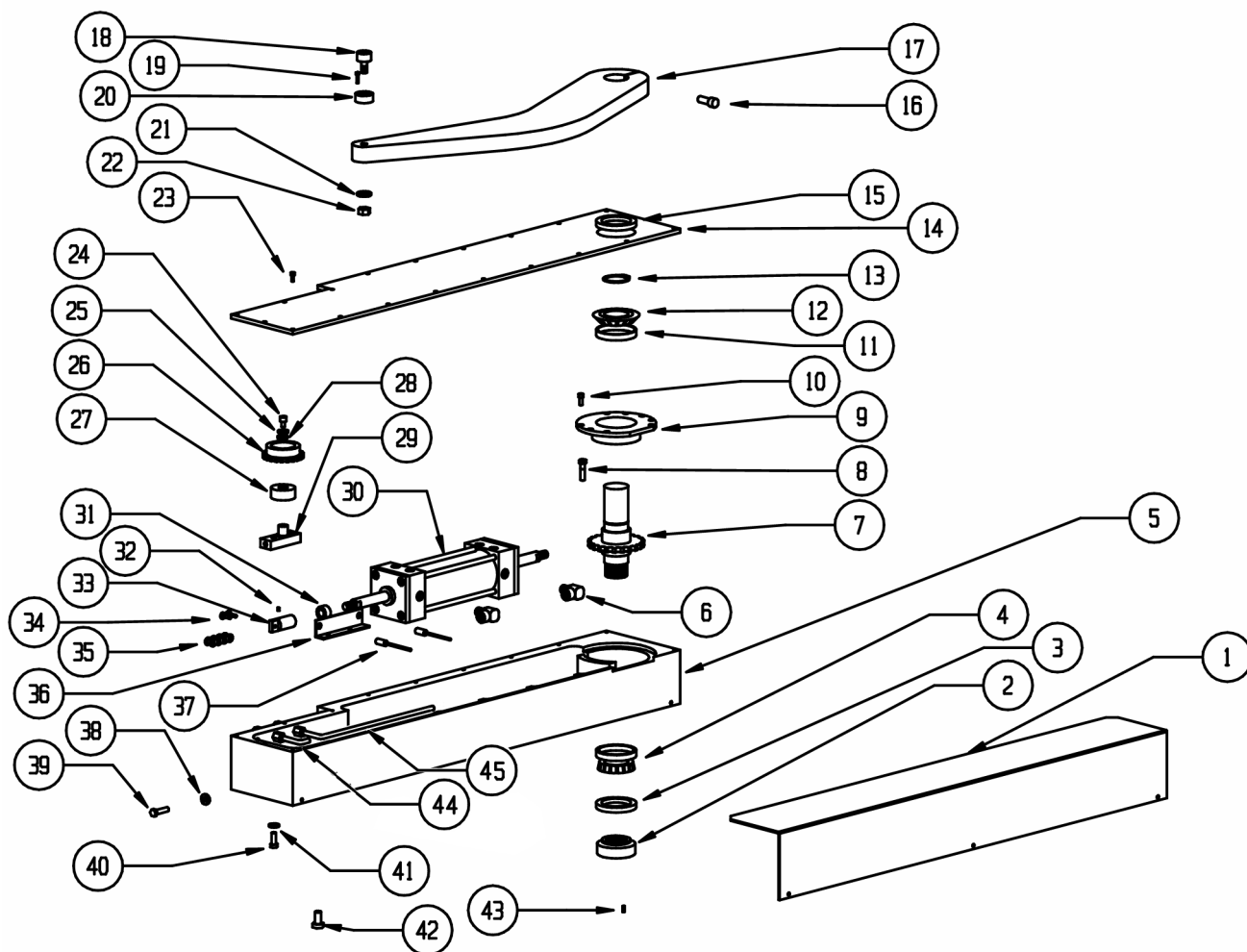
PALLET CHANGER
