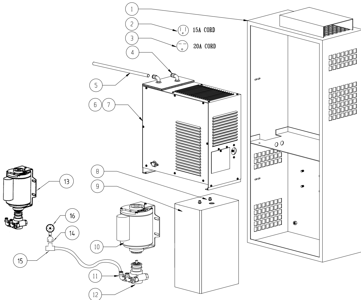
CHILLER CABINET ASSEMBLY
