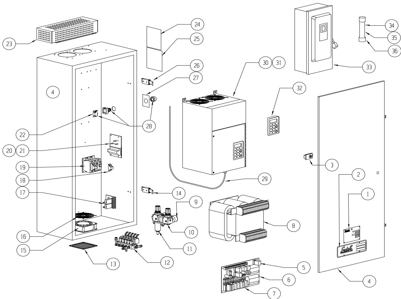
POWER JUNCTION CABINET ASSEMBLY
